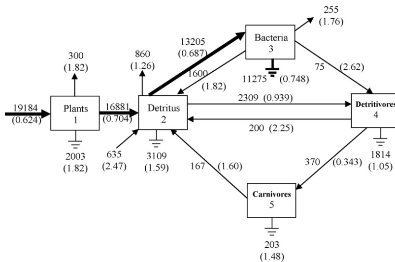
Fig. 6 – The Cone Spring network, as in Fig. 5, except that 8000 \text{ kcal m}^{-2} \text{y}^{-1} has artificially been added over the route, 1 \rightarrow 2 \rightarrow 3 . Corresponding changes in the increments at the margin are shown in parentheses.
